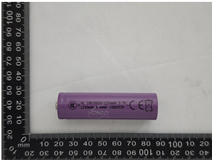
Figure 4 Side view of cell (IMR18650-1200mAh)
