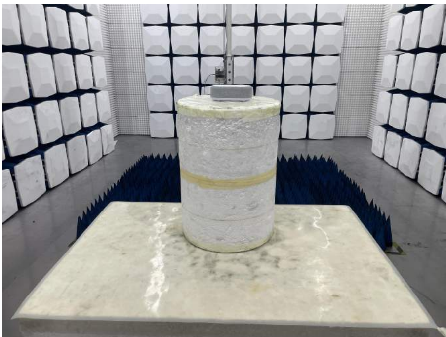
Radiated Emission Test Setup 2 1 GHz - 12.75 GHz (Transmitter tests)
